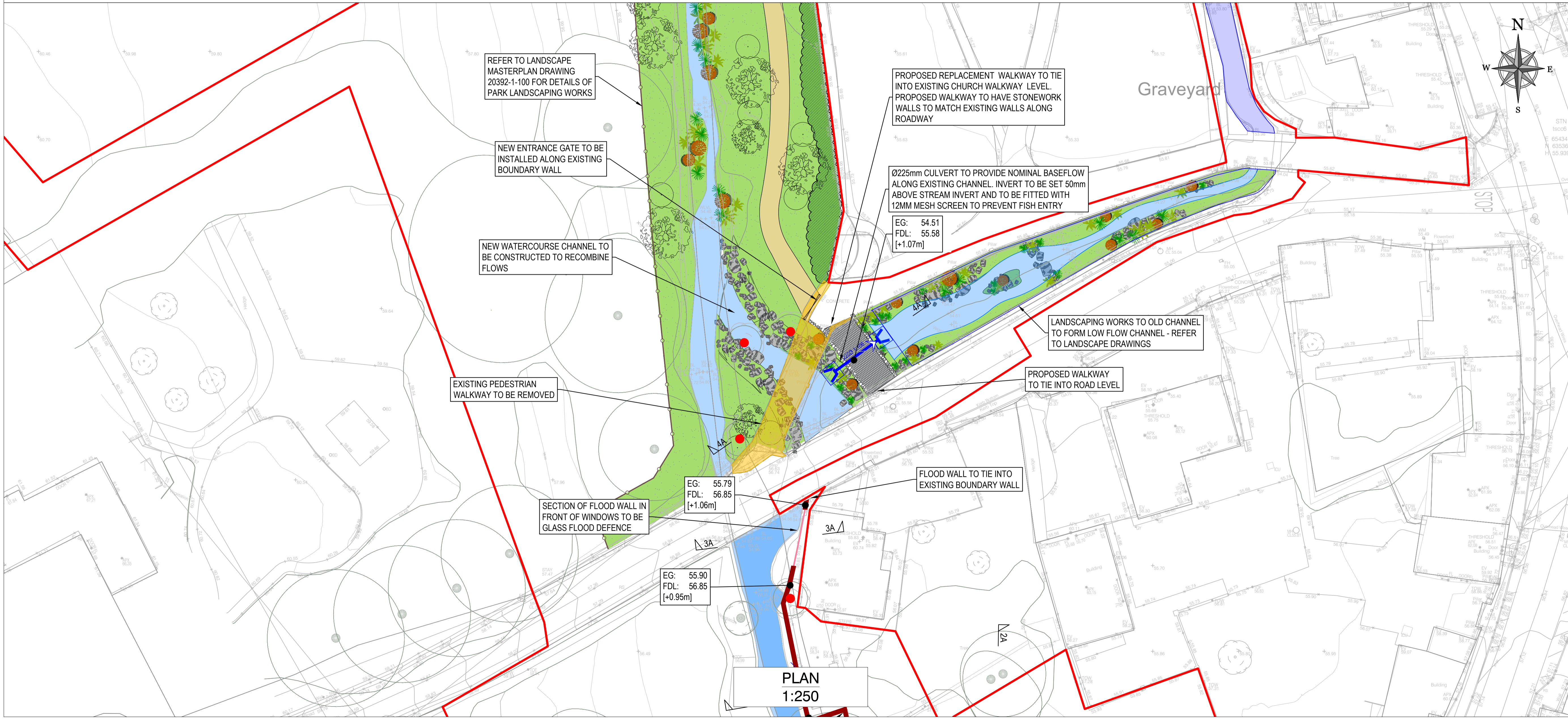
SECTION 1:50
