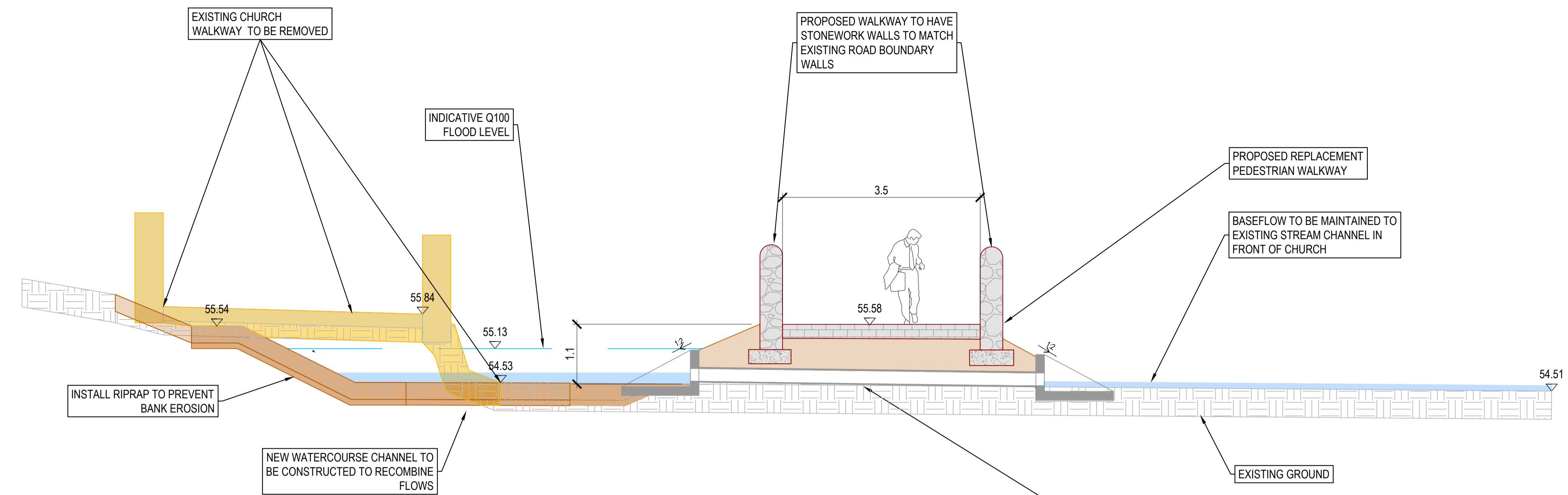
E-003 / D-001 CROSS SECTION 4A-4A
